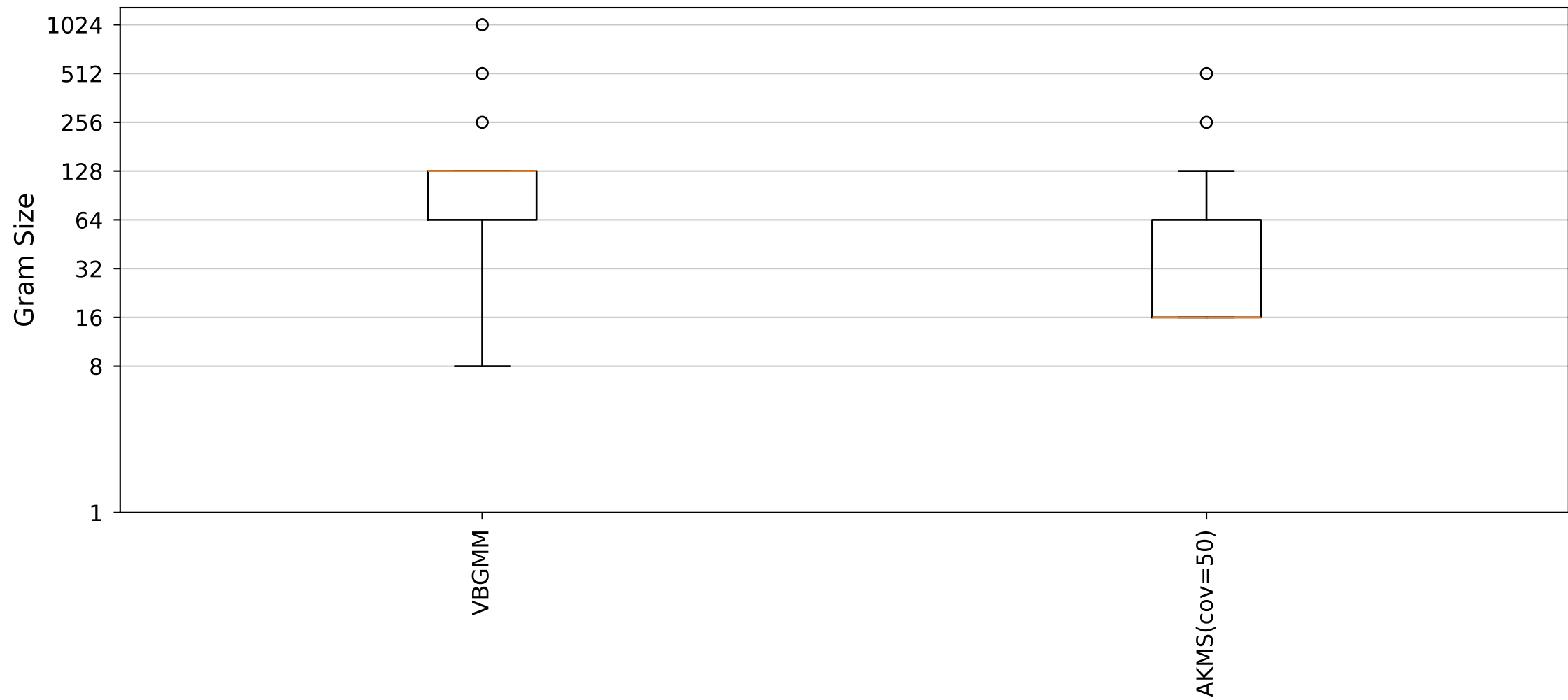
YARA Rules Gram Size Distribution (Cluster10_Size10 dataset)
